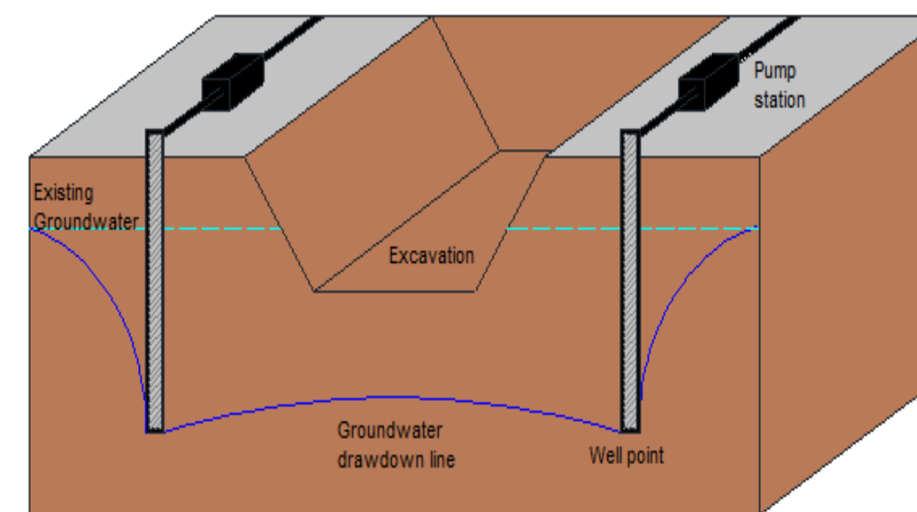
Site dewatering cross section
