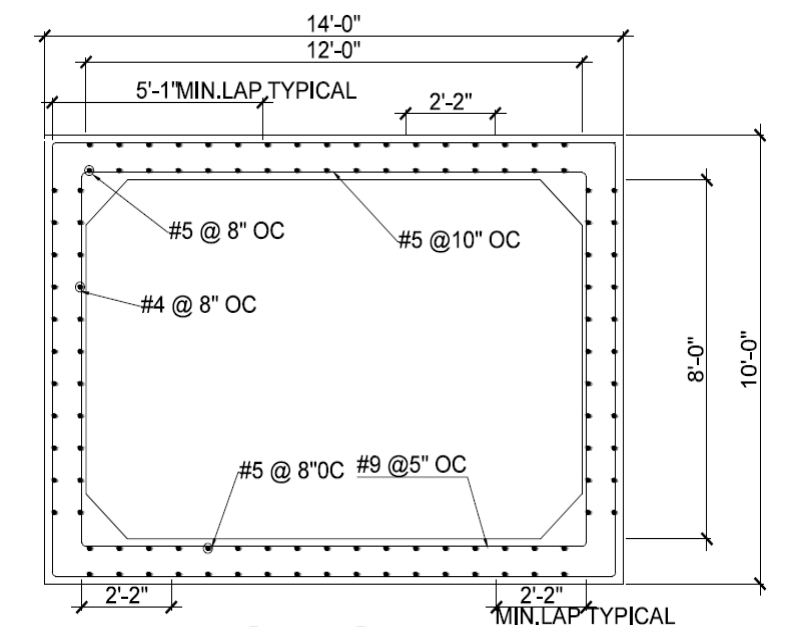
Typical box culvert section, with rebar detail.
