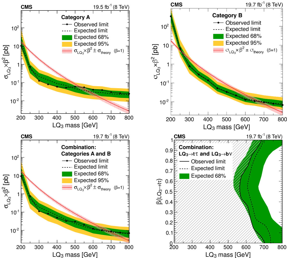
Figure 6. The expected and observed exclusion limits at 95% CL on the LQ 3 pair production cross section times \beta^2 in category A (upper left), category B (upper right) and the combination of the two categories (lower left). The theoretical uncertainty in the LQ pair production cross section includes the PDF and renormalization/factorization scale uncertainties as prescribed in ref. [19]. The expected and observed limits on the LQ branching fraction \beta as a function of the LQ mass (lower right). The total excluded region (shaded) is obtained by including the results in ref. [17], reinterpreted for the LQ 3 → bν scenario.
